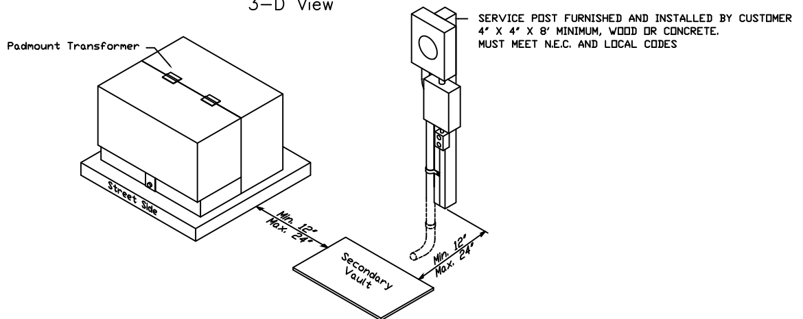
TRANSFORMER + SECONDARY VAULT 3-D View
